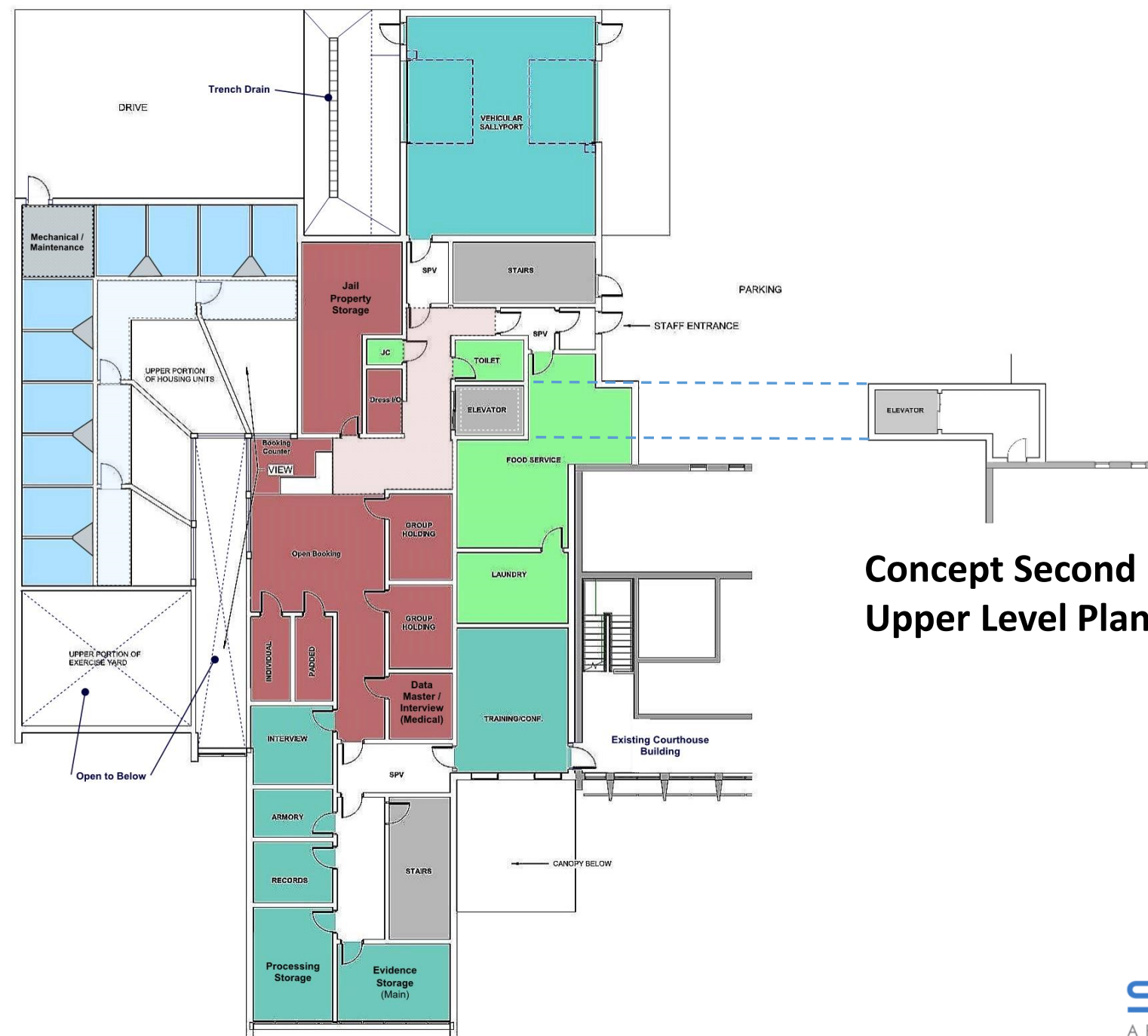
Concept First Floor – Upper Level Plan
